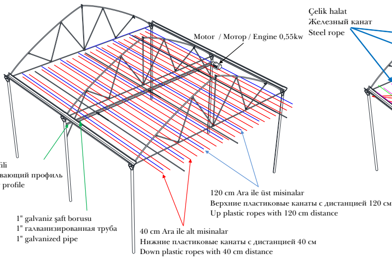
PUSH PULL PERDE SİSTEMİ PUSH PULL SHADING SYSTEM СИСТЕМА ЗАШТОРИВАНИЯ PUSH PULL
